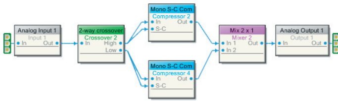
Figure 8. Drag Net split-band processing.
