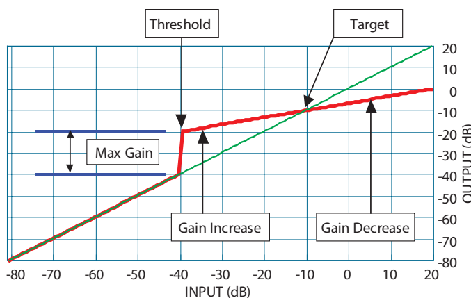
Figure 13b. AGC response graph.
