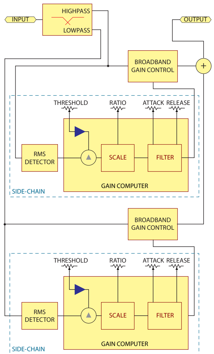
Figure 7. Split-band compressor block diagram.
