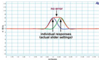
Figure 3: Elimination of band interaction in Perfect-Q.
